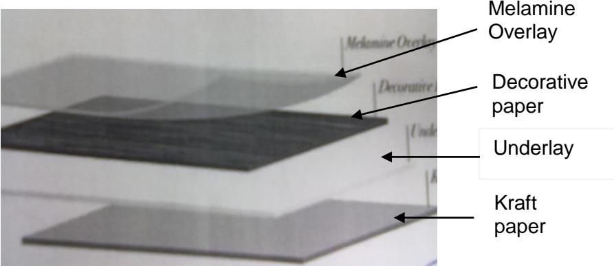
Gambar komposisi High pressure Laminates(HPL)
