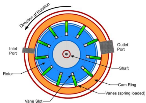
Keratan rentas Vane-type hydraulic motor M5B* Series
