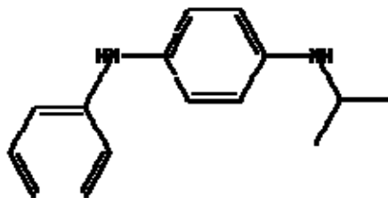
N-Isopropyl—N'-phenyl-p-phenylenediamine
